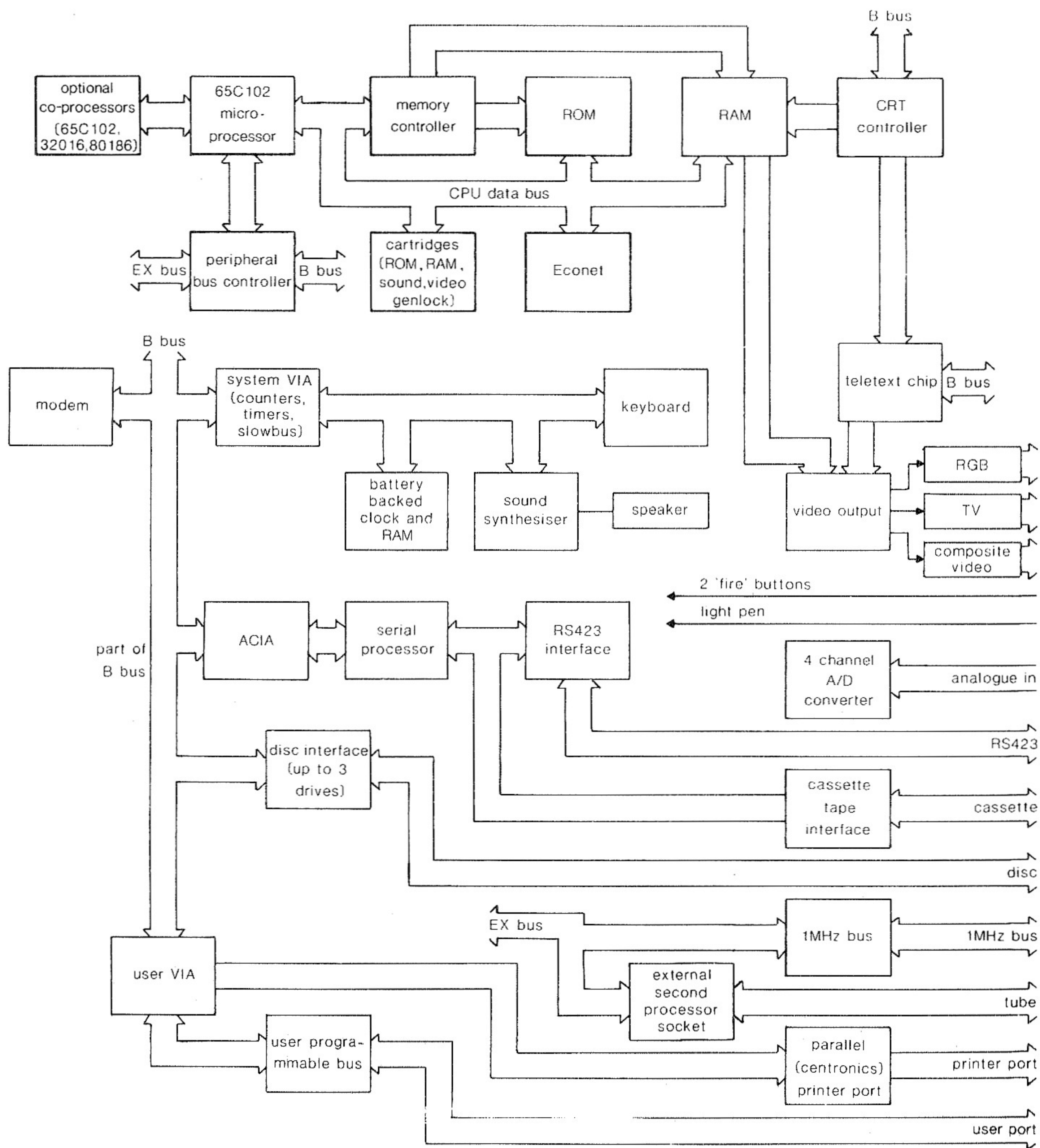
System block diagram
